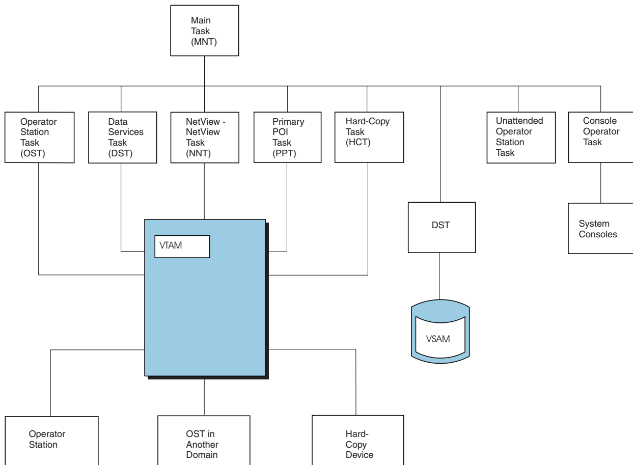
Figure 5. Structural Overview of the Command Facility
